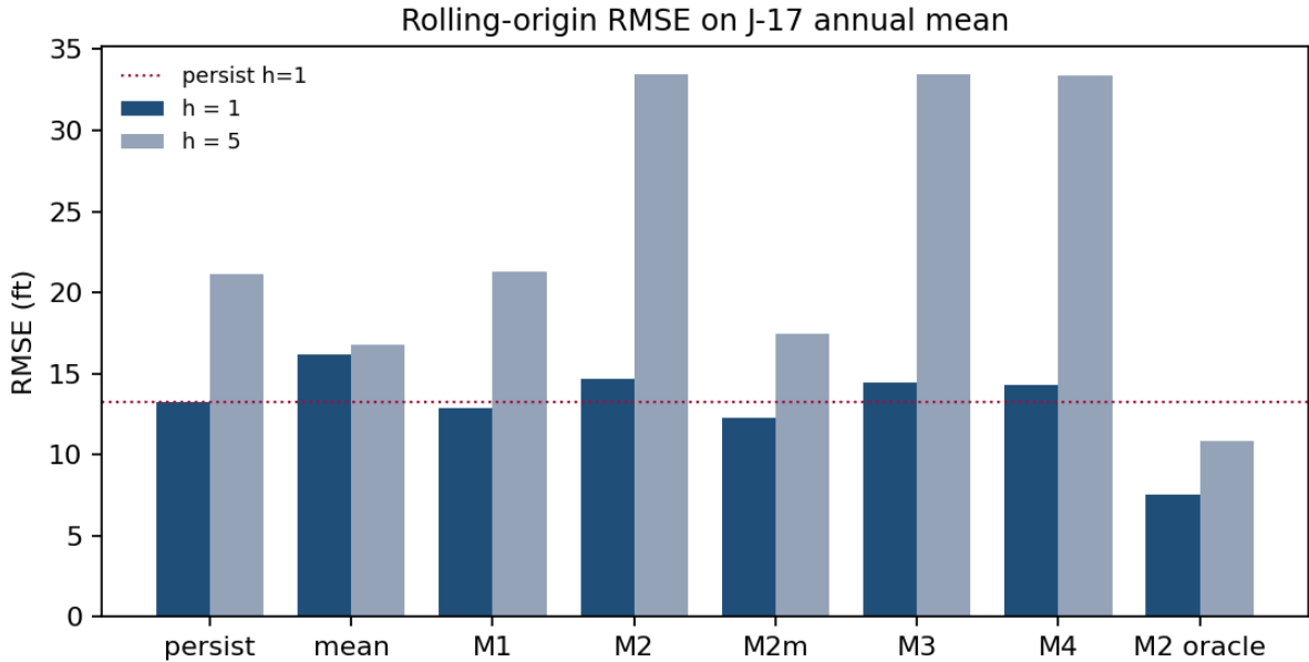
Figure 9: Rolling-origin RMSE. The oracle is excluded from retention.
