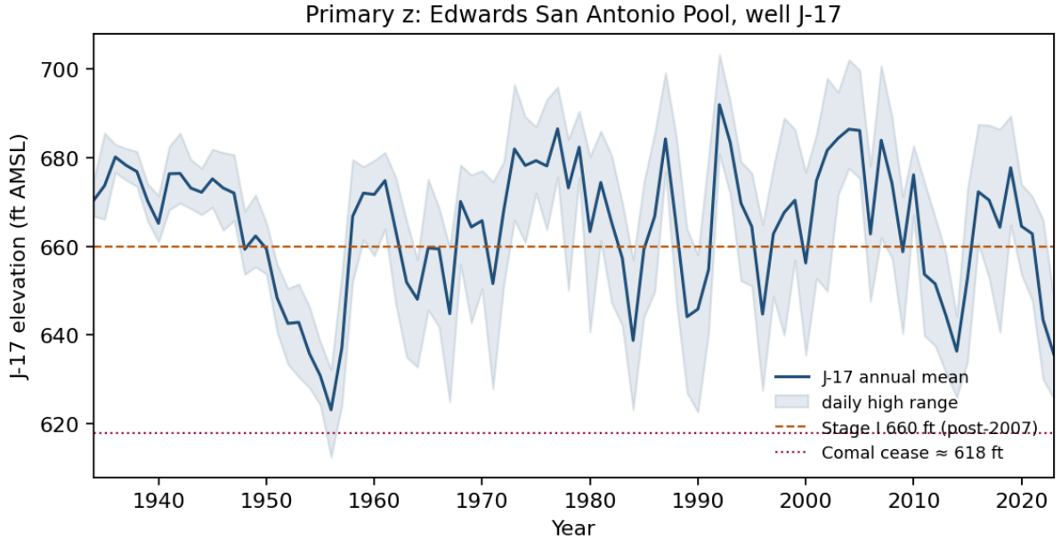
Figure 7: J-17 annual mean and daily-high range. 1956 mean 623.15 ft, daily minimum 612.51 ft. 1992 mean 691.96 ft, daily maximum 703.31 ft. 2023 mean 635.68 ft. The annual mean is below 660 ft in 31 of 90 years; the daily minimum is below 618 ft in one year (1956).
